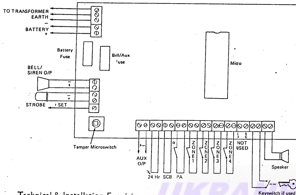
PCB LAYOUT
