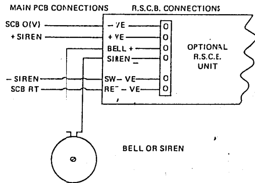
DIAGRAM SHOWING CONNECTION OF R.S.C.B.
